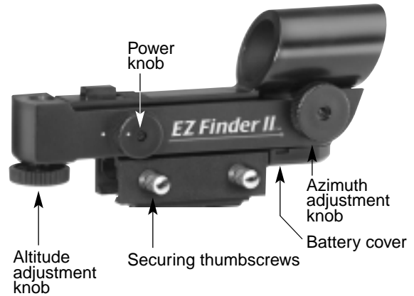
Figure 3. The EZ Finder II reflex sight.
