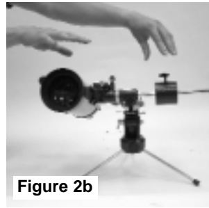
Figure 2a, b. Proper operation of the equatorial mount requires balancing the telescope tube on the R.A. axis. (a) With the R.A. lock knob released, slide the counterweight along the counterweight shaft until it just counterbalances the tube. (b) When you let go with both hands, the tube should not drift up or down.
