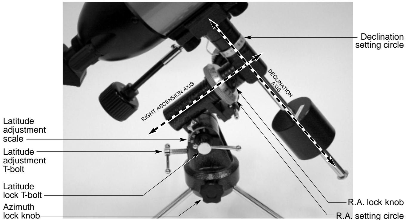
Figure 4. The Transporter 70 Min-EQ equatorial mount.
